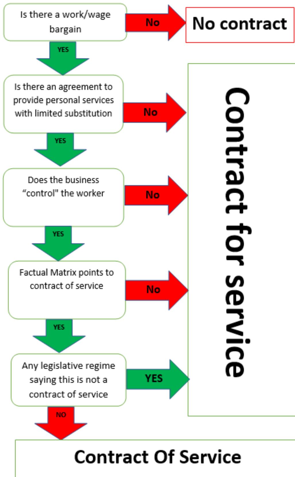
Figure 1: Decision Tree
