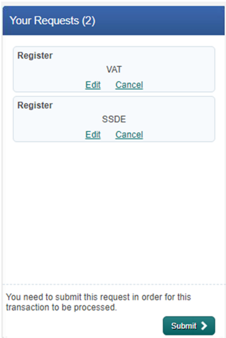
Figure 10: Cart Screen
