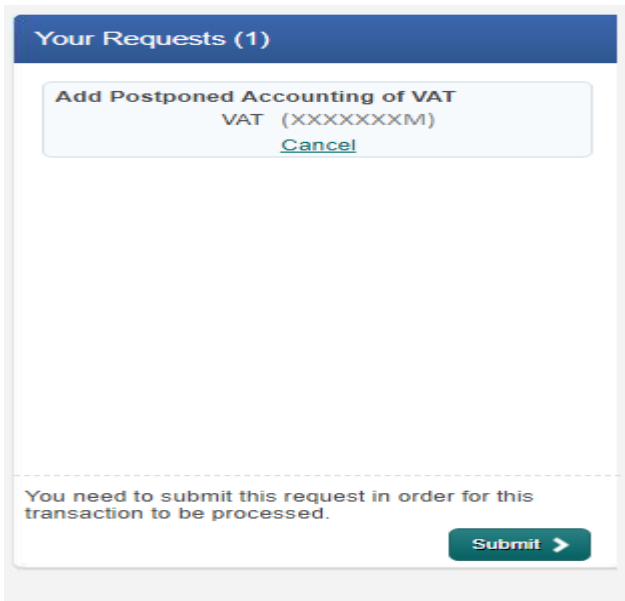
Figure 21: Submit request
